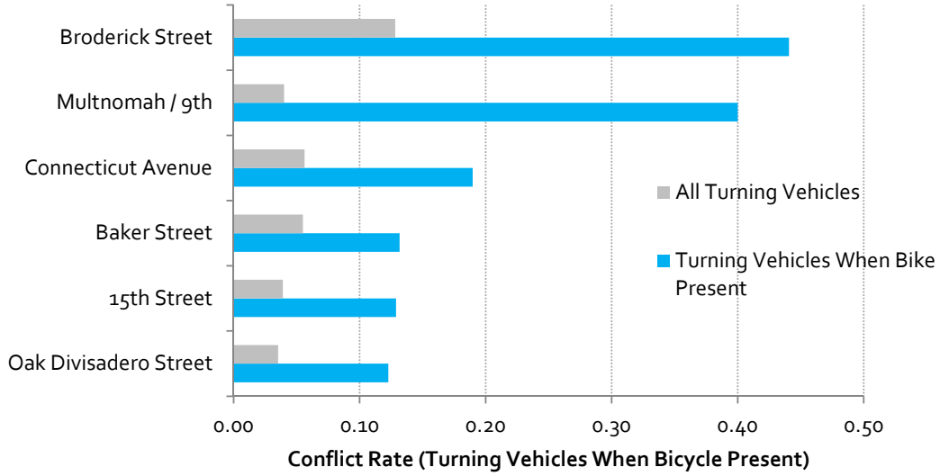
Figure 8-6. Comparison of Conflict Rates at Intersections
