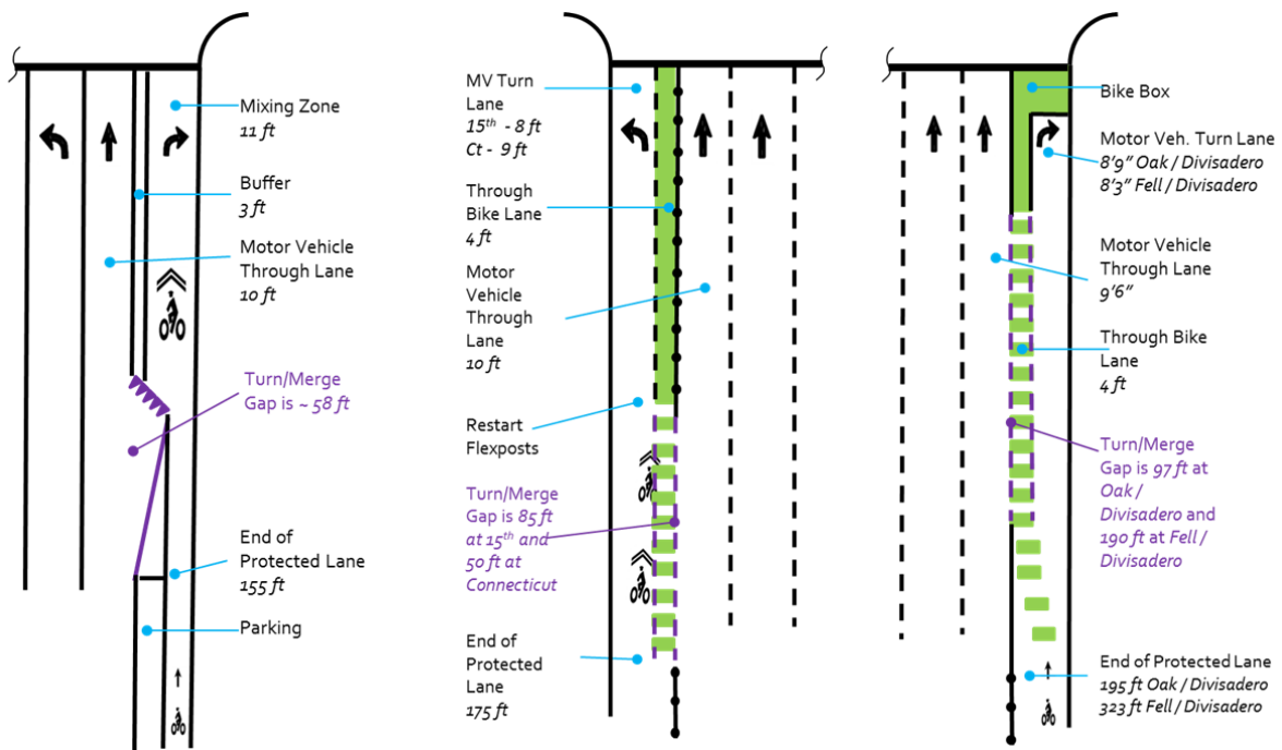
Mixing Zone with Yield Entry Markings NE Multnomah and NE 9 th Ave
