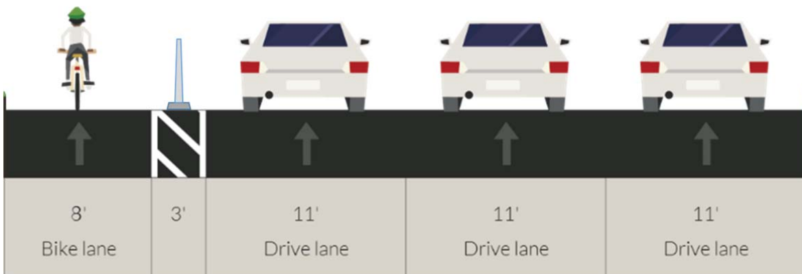
Figure 3-38. Sample cross section of L Street Protected Bike Lane
