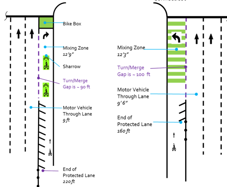
Mixing Zone with Sharrow Oak St. and Broderick St
