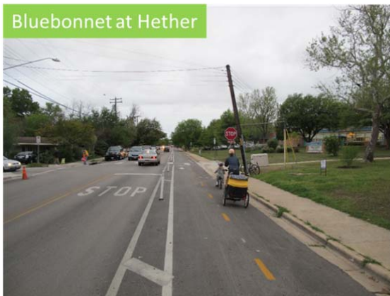
Figure 3-9. Bluebonnet Lane Protected Bike Lanes, Austin, TX
