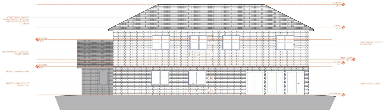
2 WEST ELEVATION Scale: 1/4" = 1'-0"
