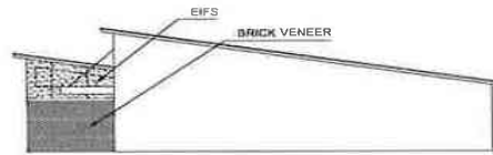
RECESS ELEVATION — SCALE: 1/8"=1'-0"
