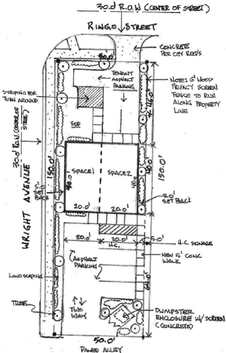
SITE PLAN OF PROPOSED DEVELOPMENT
